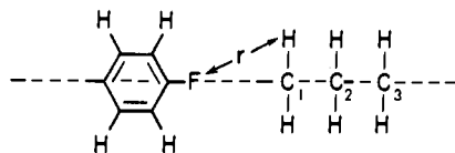
Figure 1. Structure of the 11 spin \frac{1}{2} nuclei model used in the calculations described in the text. The internuclear distances in the left array were those of a p -fluorophenyl group. All distances were held fixed for the calculations except r .
