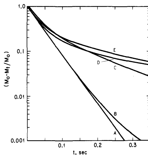
Figure 6. Computed spin-lattice relaxation curves when r = 2.0 \text{ \AA} in the model system and \tau_c = 1.67 \times 10^{-8} \text{ s} . Curve A is for the fully decoupled system where strictly exponential relaxation is expected while curve E is for the fully coupled situation. Curves B, C, and D represent the computed relaxation behavior upon selective irradiation of methylene groups 1, 2, and 3, respectively.
